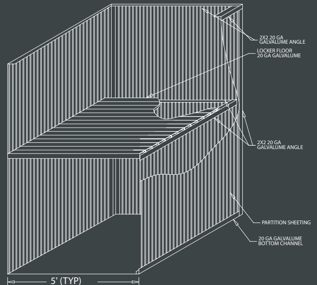
LOCKER FLOOR DETAIL
