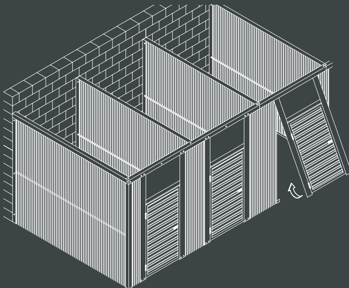
CORRUGATED SWING DOOR DETAIL
